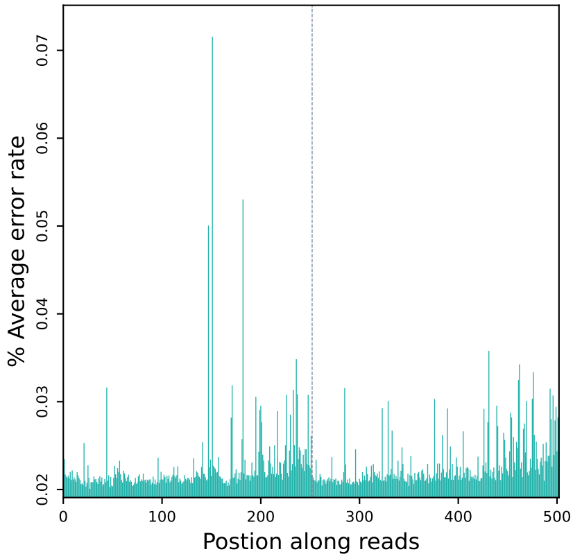
Error rate distribution along reads (R10727)
